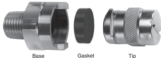
EZNF exploded
