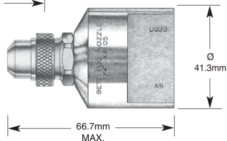
Overall Dimensions for Assemblies with XA05 Bodies
