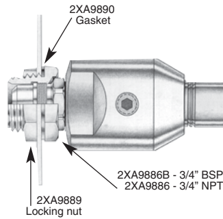
XA02 with Thin Wall 02 Adapter
