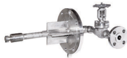
WTZ Lance with Inlet Valve and Gussets
