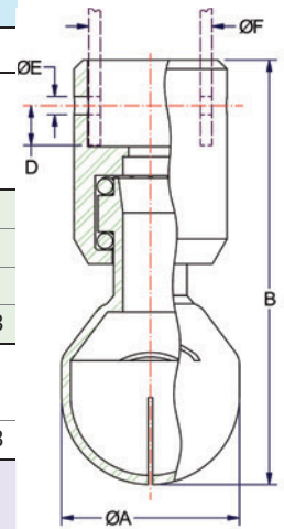
Threaded and Clip On Connections
