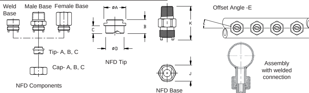
NFD Base
