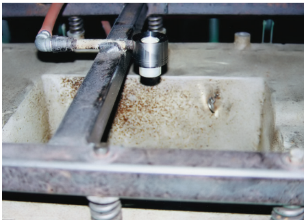
A Model 121021 1-1/4" (32mm) High Temperature Air Amplifier directs hot air to a rotational mold cavity for uniform wall thickness of the plastic part.
