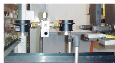
(2) Model 120022 2" (51mm) Super Air Amplifiers dry small parts as they move down along a parts conveyor.
