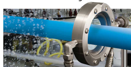
The stainless steel Super Air Wipe is ideal for food and pharmaceutical applications.
