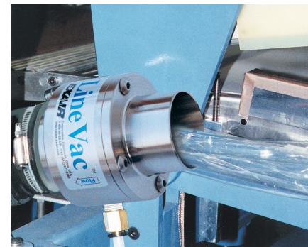
A Model 6084 2" (51mm) Line Vac transports scrap cellophane trim to a waste barrel.
